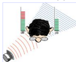
Interaural Level Difference (ILD)
